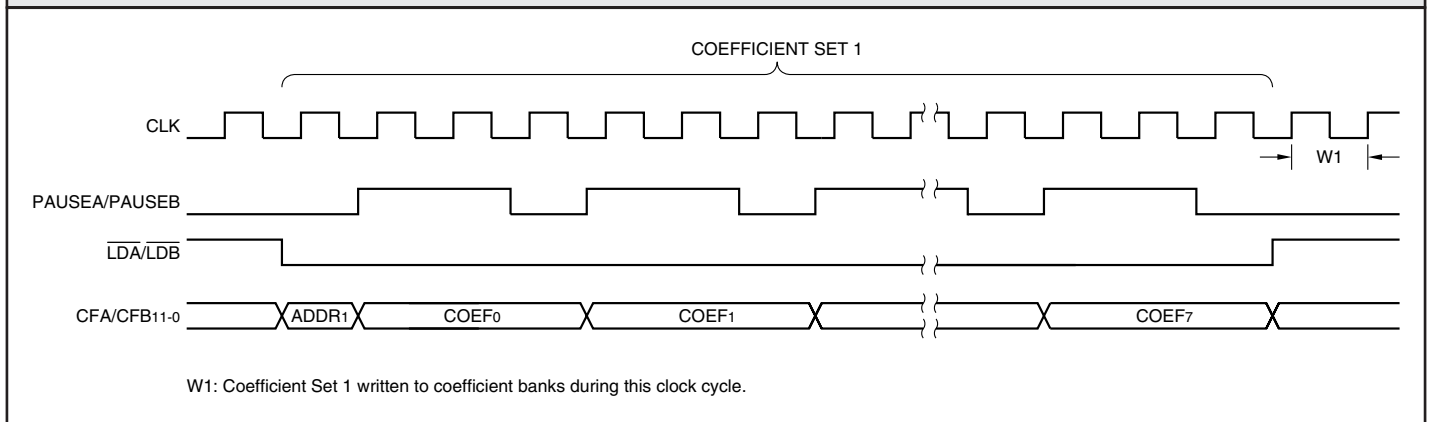
FIGURE 19. COEFFICIENT BANK LOADING SEQUENCE WITH PAUSE IMPLEMENTATION
